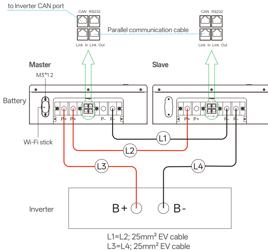
Scheme One (Inverter Power \leq 5KW )
